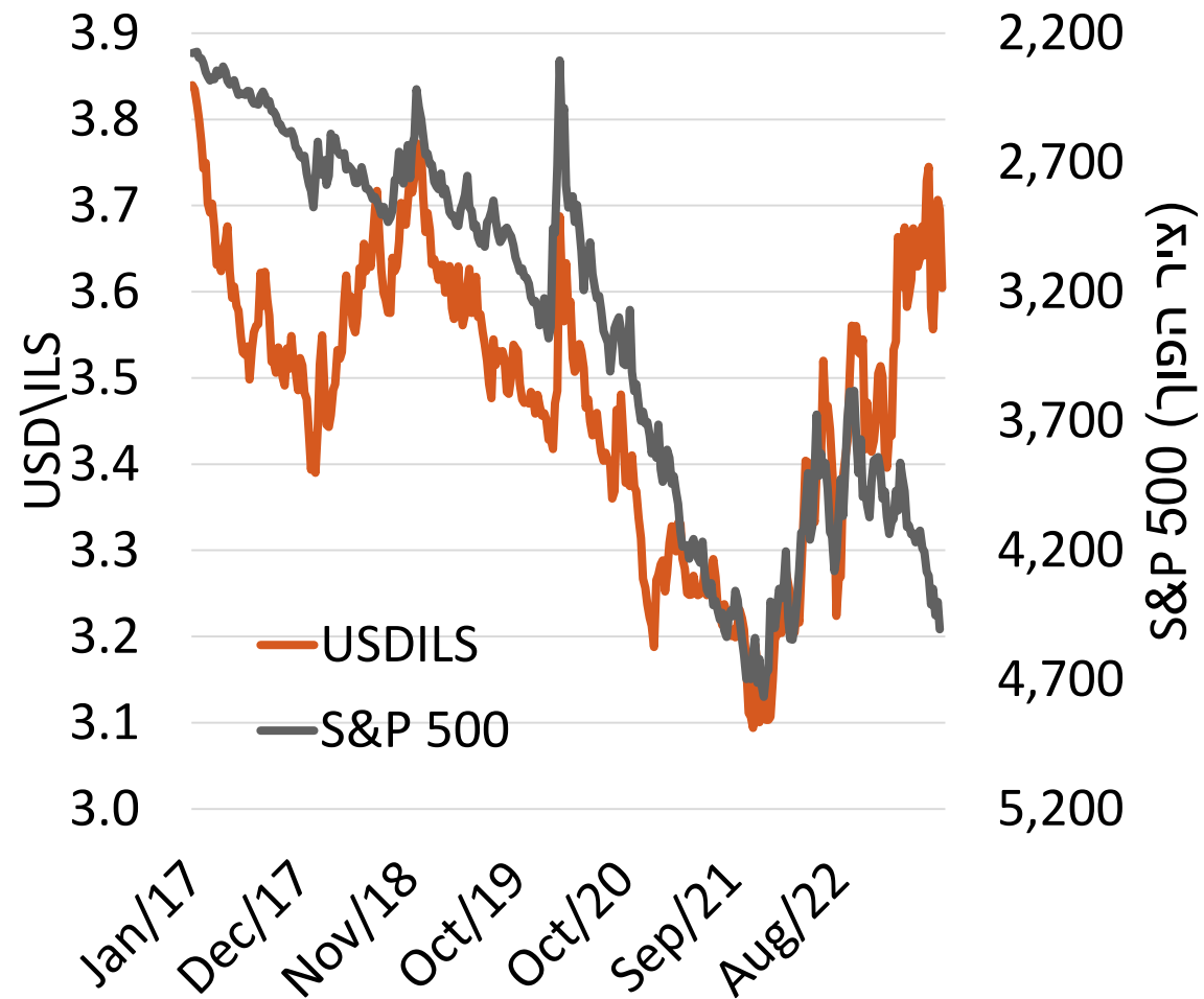
USD\ILS vs. S&P 500
