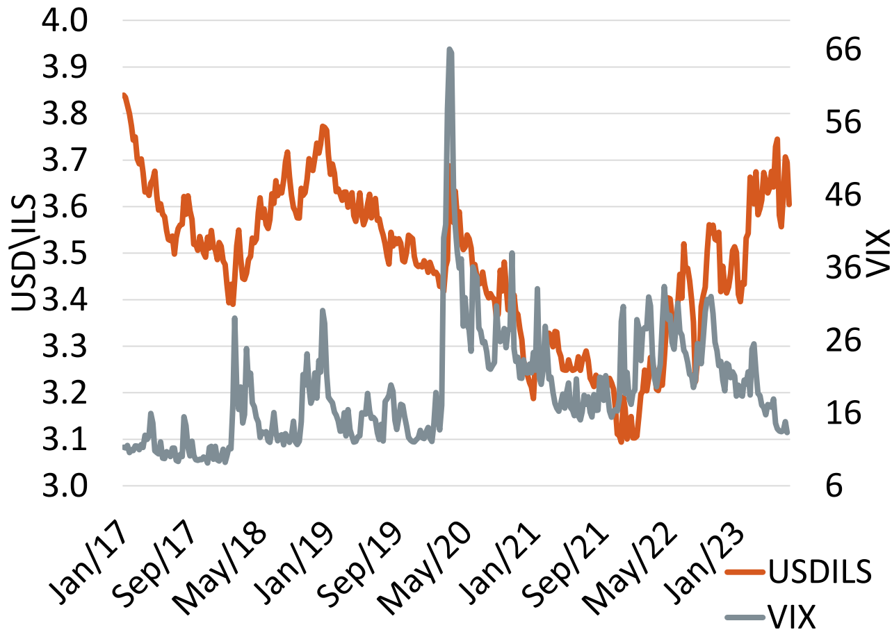
USD\ILS vs. VIX
